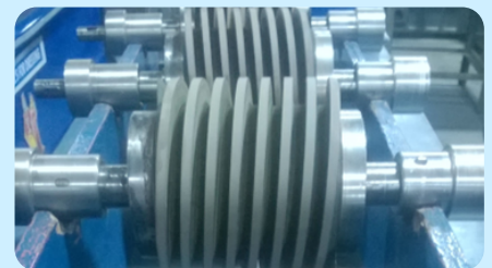
Spiral Wheel (Semi-Finish)
