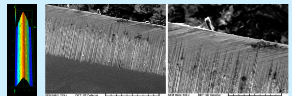
Two Faceted Blade Edge under 1000x magnification before Honing
