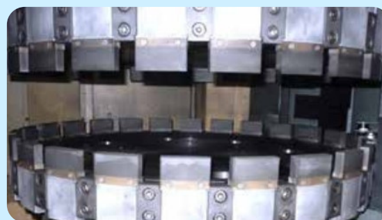
cBN Segmented Wheel for Break Disc Grinding (Uncoated / Coated)
