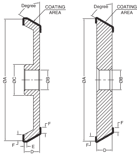
WHEEL NO. - 1
